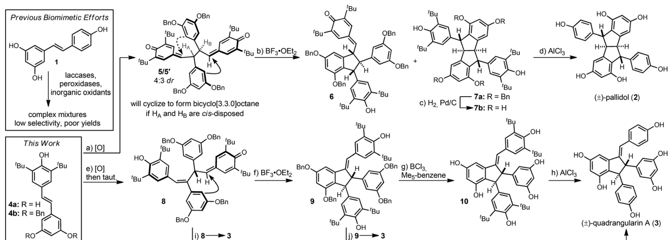
Scheme 1. The total synthesis of pallidol ( 2 ) and quadrangularin A ( 3 ): a) KHMDS (1.05 equiv), [\text{FeCp}_2]\text{PF}_6 (1.05 equiv), THF, 0 °C, 30 min, 95 %; b) \text{BF}_3 \cdot \text{OEt}_2 (2 equiv), \text{CH}_2\text{Cl}_2 , –78 °C, 40 min, 88 %, 6/7a ca. 1:1; c) Pd/C (30 wt %), \text{H}_2 (1 atm), 3:2 EtOAc/MeOH, RT, 12 h, 95 %; d) \text{AlCl}_3 (12 equiv, 2.25 M in \text{CH}_3\text{NO}_2 ), toluene, 60 °C, 30 min, 80 %; e) KHMDS (1.05 equiv), [\text{FeCp}_2]\text{PF}_6 (1.05 equiv), THF, 0 °C, 30 min, then KHMDS (1.25 equiv), 15 min; f) \text{BF}_3 \cdot \text{OEt}_2 (2 equiv), \text{CH}_2\text{Cl}_2 , –78 °C, 5 min, 90 % over 3 steps; g) \text{BCl}_3 (12 equiv), \text{Me}_5\text{-benzene} (20 equiv), \text{CH}_2\text{Cl}_2 , –78 °C, 2 h, 82 %; h) \text{AlCl}_3 (12 equiv, 2.25 M in \text{CH}_3\text{NO}_2 ), toluene, 60 °C, 30 min, 80 %; i) \text{Me}_5\text{-benzene} (40 equiv), \text{AlCl}_3 (25 equiv, 0.6 M in \text{CH}_3\text{NO}_2 ) slow addition, \text{CH}_2\text{Cl}_2 , 0 °C, then 60 °C, 15 min, 51 %; j) \text{Me}_5\text{-benzene} (40 equiv), \text{AlCl}_3 (24 equiv, 0.5 M in \text{CH}_3\text{NO}_2 ) slow add'n, \text{CH}_2\text{Cl}_2 , 0 °C, then 60 °C, 1 h, 88 %, 5:1 mixture of quadrangularin A ( 3 ) to its internal alkene isomer. Bn = benzyl, t Bu = tert -butyl, taut. = tautomerization, KHMDS = potassium hexamethyldisilazide, [\text{FeCp}_2]\text{PF}_6 = ferrocenium hexafluorophosphate, THF = tetrahydrofuran, \text{Me}_5\text{-benzene} = pentamethylbenzene.
